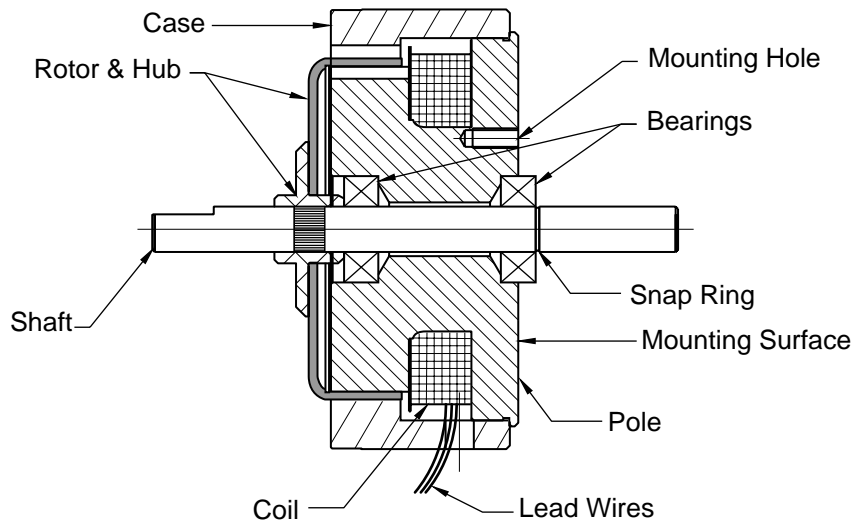
Figure 1. Hysteresis Brake
