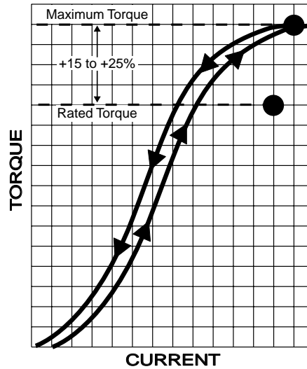
Figure 3. Torque/Current Curve
