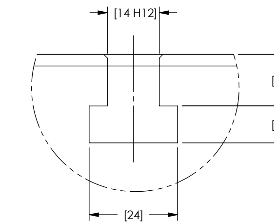
DETAIL B SCALE 1 : 1 7X M14 H12 T-SLOT
