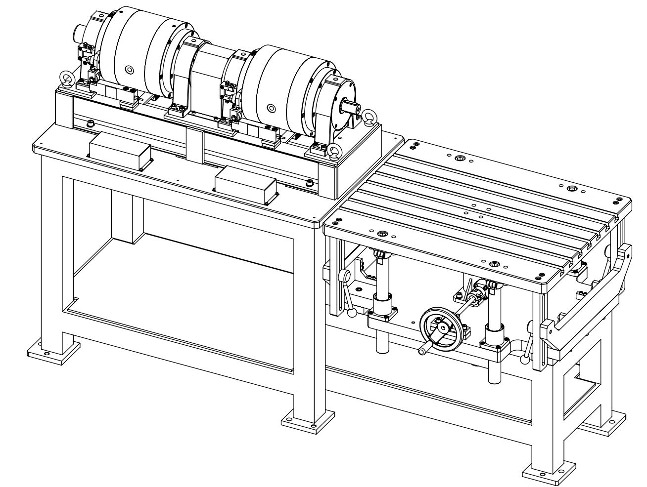
3 DIMENSIONAL VIEW SCALE 1 : 12
